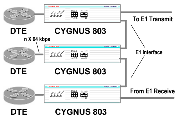
Fig. 2 Multiple units cascaded to allow several DTEs to access a single framed E1 interface
